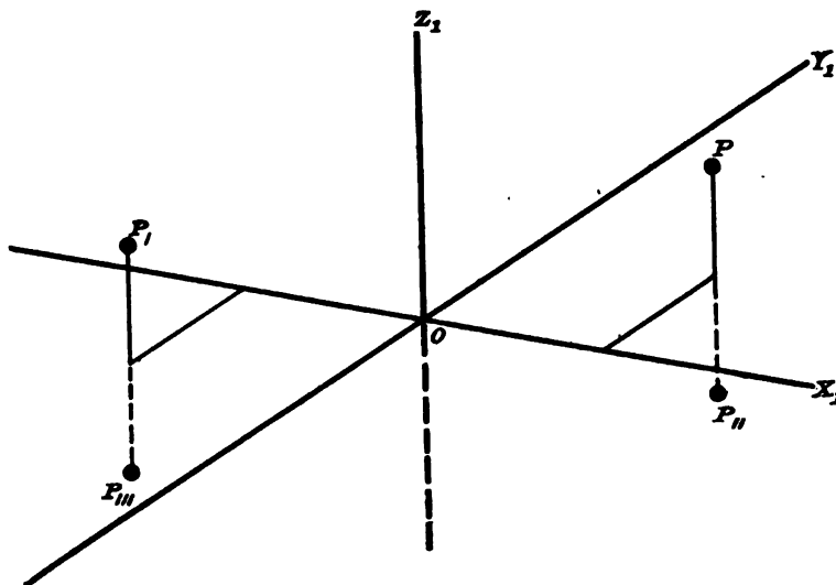
FIG. 19. The point-group C_{2h} . The points P, P', P'', P''' are the four equivalent points of this point-group.
